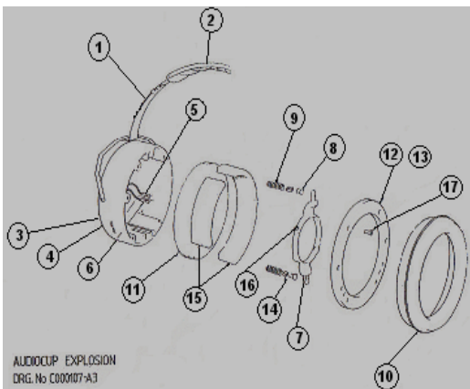
AMPLIVOX AUDIOCUP COMPLETE ASSEMBLY
